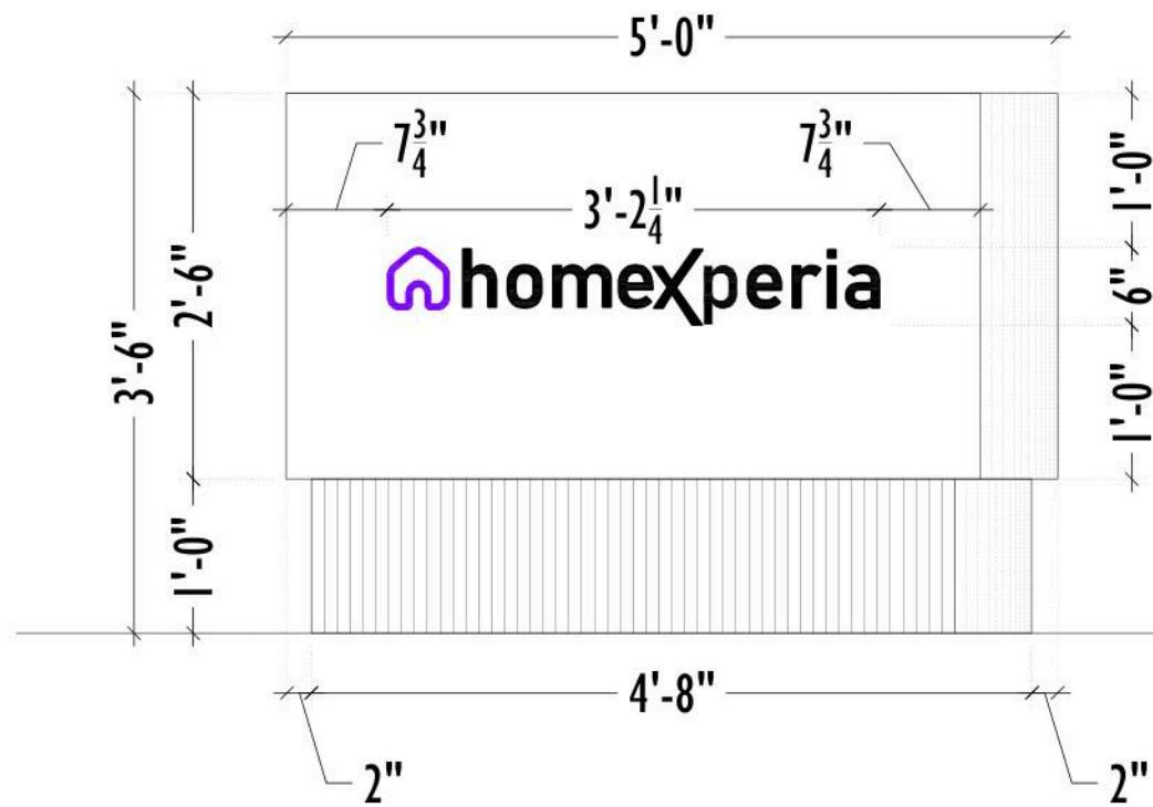
FRONT ELEVATION
